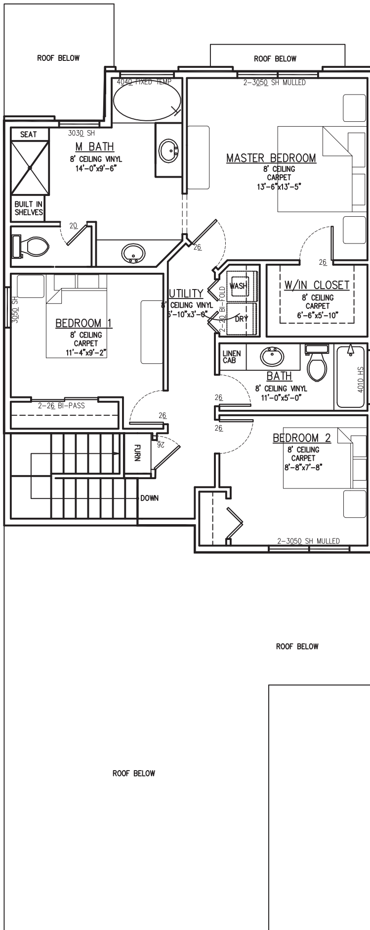
THE DESIRE _____ UPSTAIRS FLOORPLAN 1/4"=1'-0"
