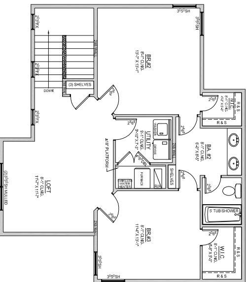
UPPER FLOOR PLAN NOT TO SCALE
