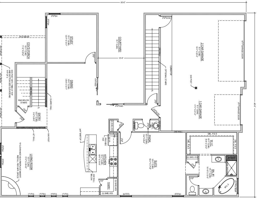
LOWER FLOOR PLAN NOT TO SCALE
